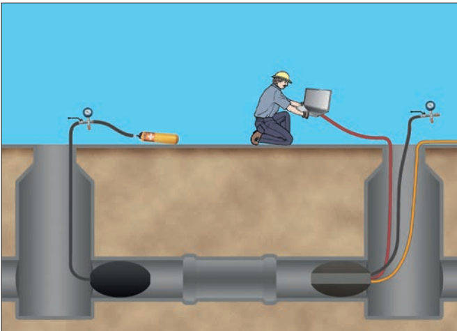
The test of leakage with air according DIN EN 1610
